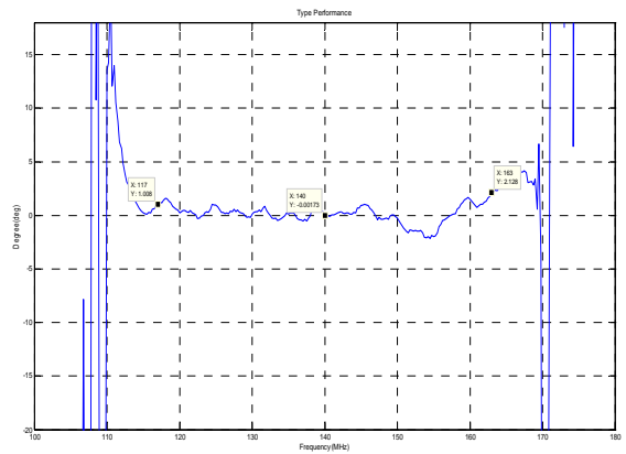
Phase Linearity(f0±23MHz)
