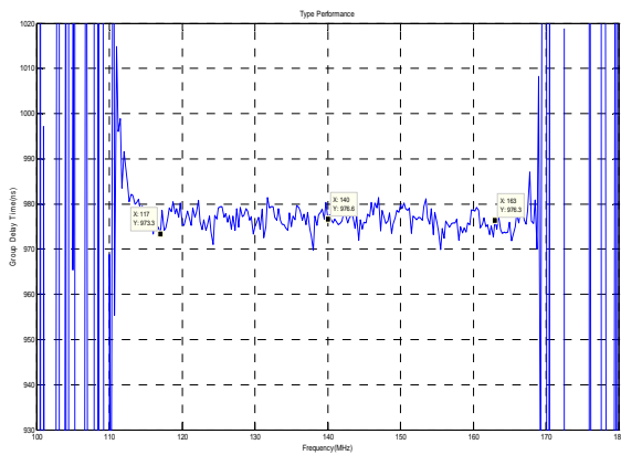
Group Delay Variation(f0±23MHz)
